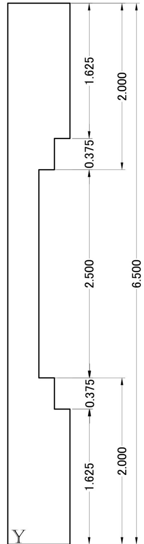
Reduced Rail
