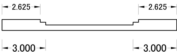
Standard Rail
