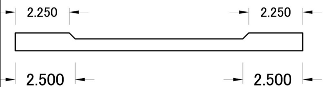
Standard Rail
