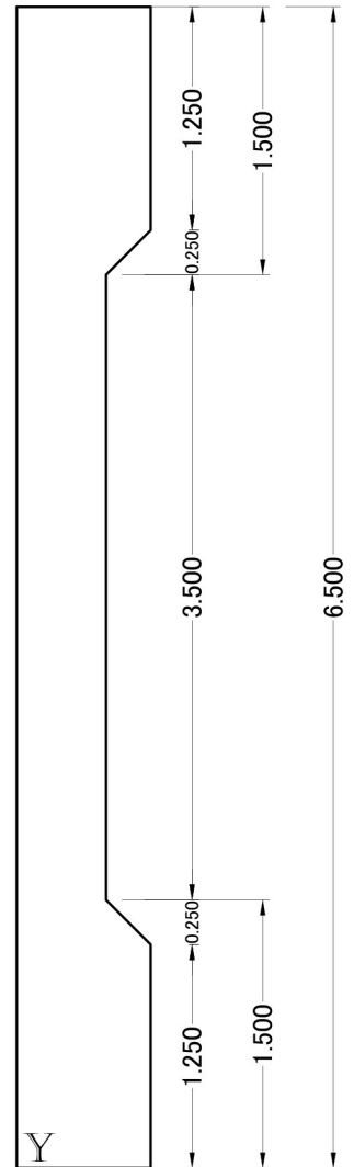
Reduced Rail
