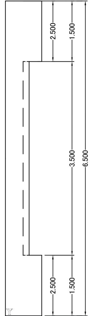
Reduced Rail
