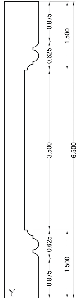
Reduced Rail
