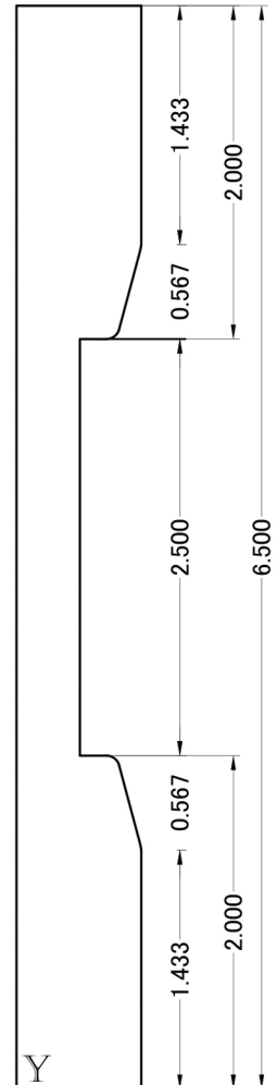
Reduced Rail
